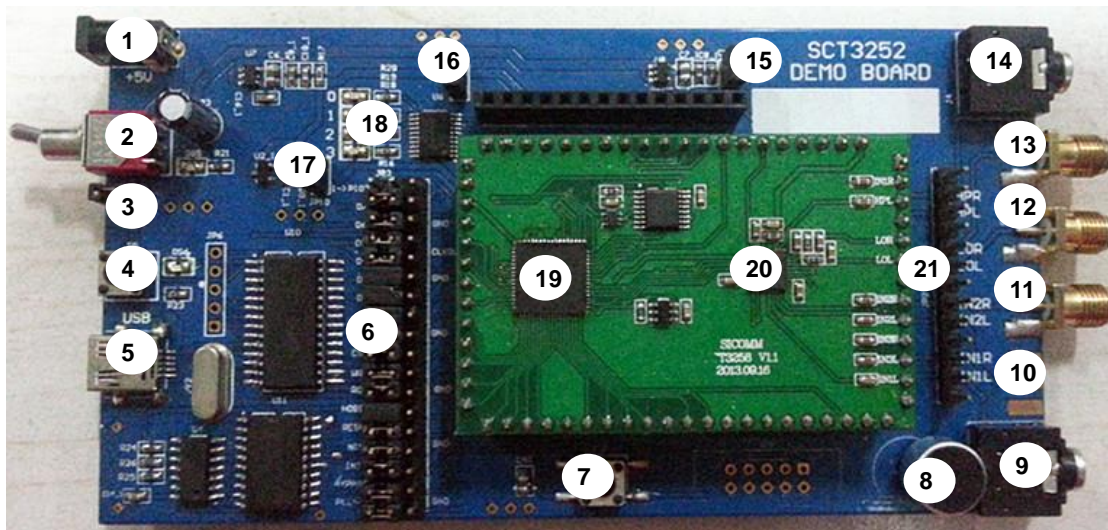
Figure 2 SCT3258 Development Board
