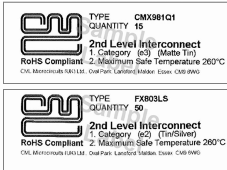
Fig 1. Example labels for Tin/Silver and Matte Tin lead terminations.
