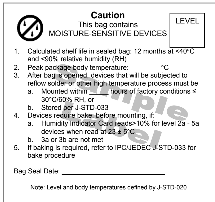
Fig 2. The Moisture-Sensitive Caution Label
