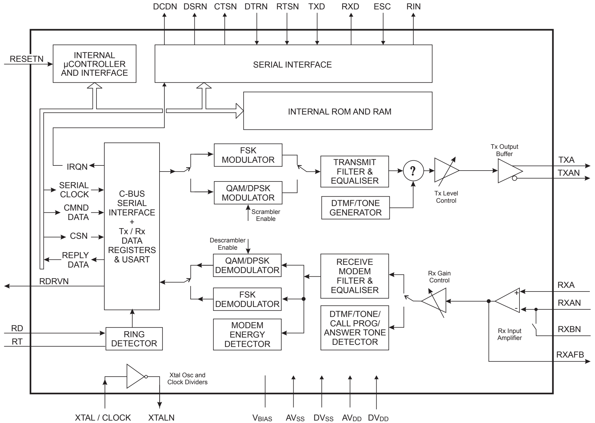
CMX866 Block Diagram
