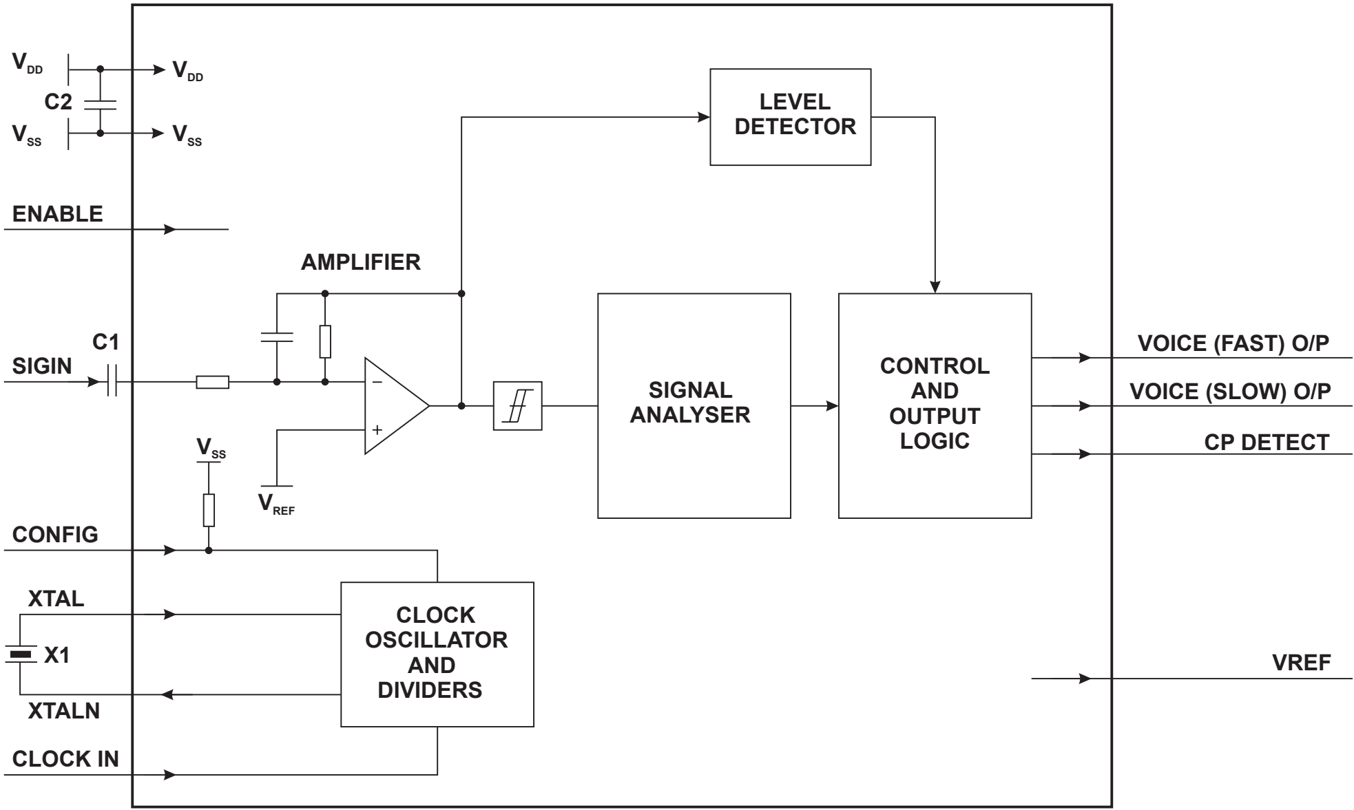
CMX683 Block Diagram
