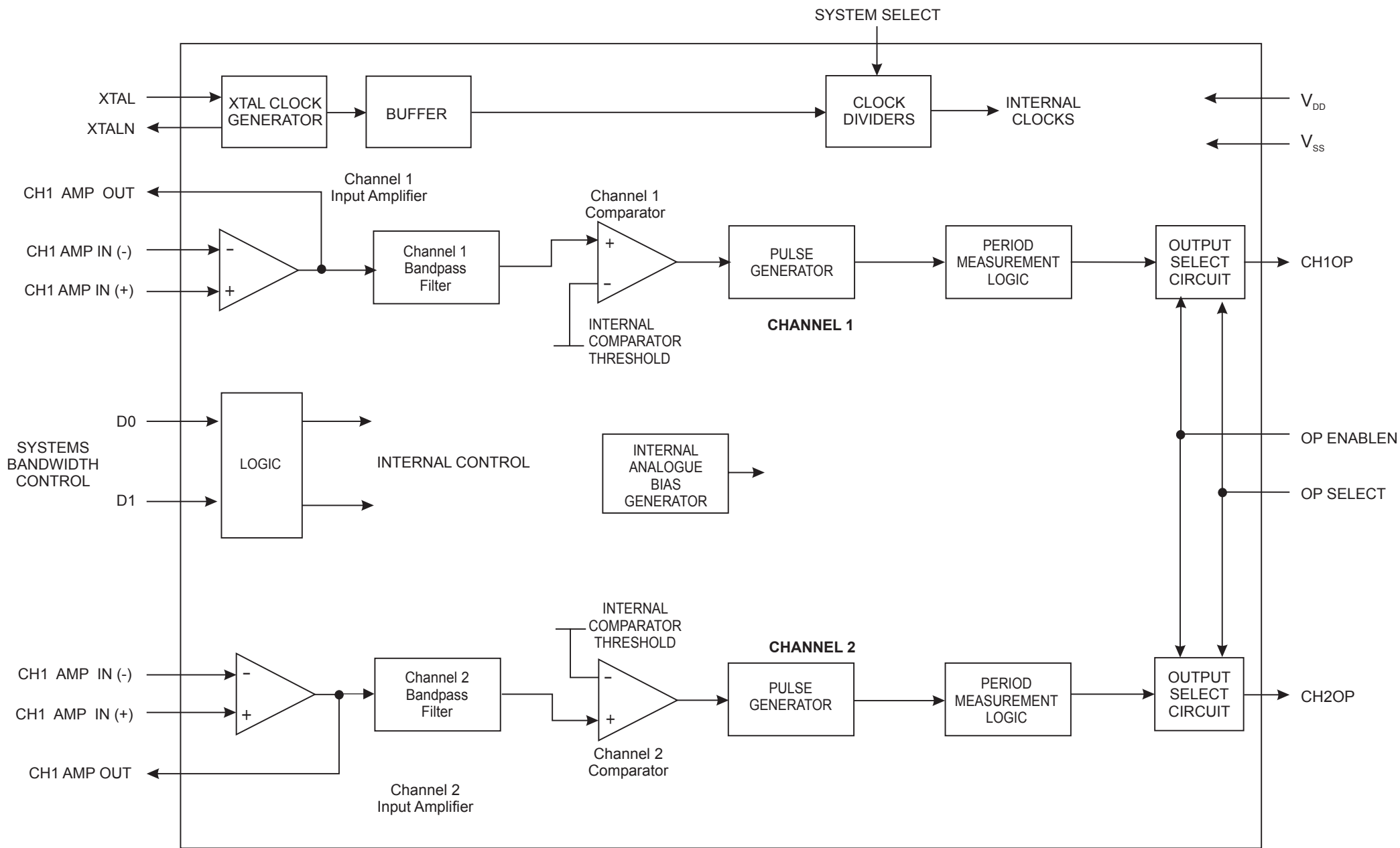
CMX661 Block Diagram
