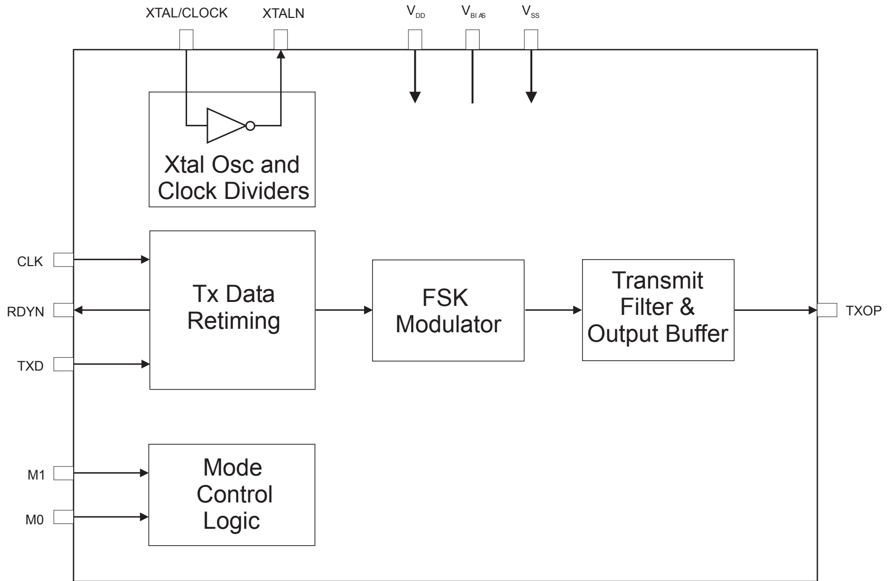
CMX654 Block Diagram
