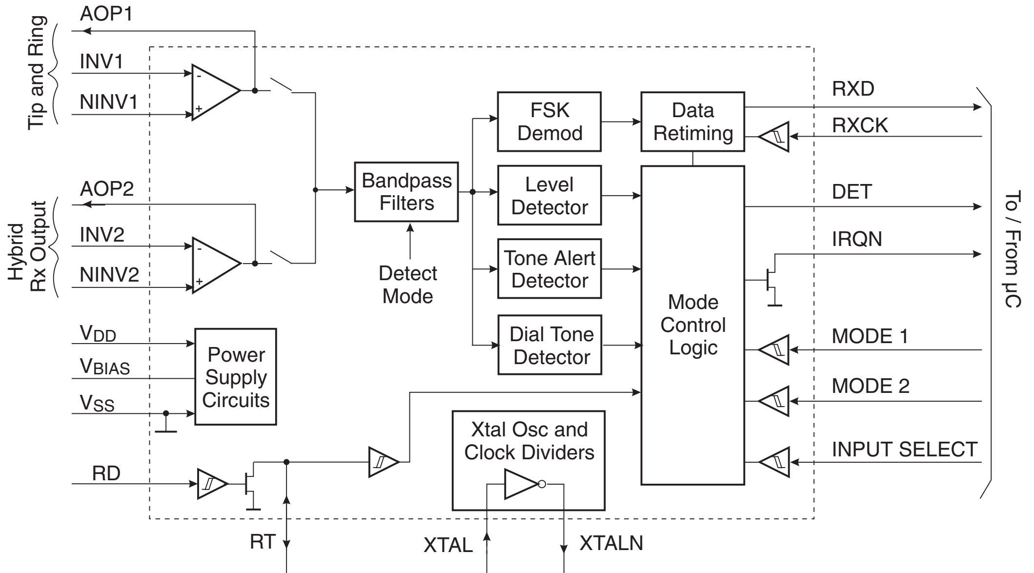
CMX612 Block Diagram
