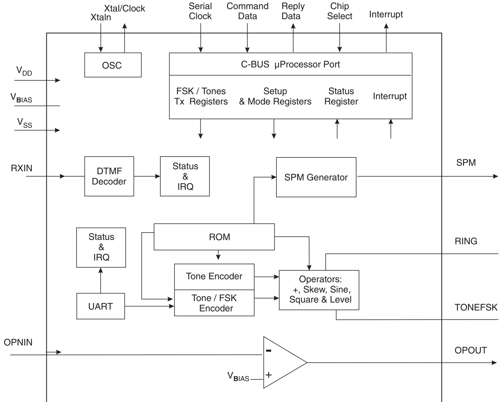
CMX605 Block Diagram
