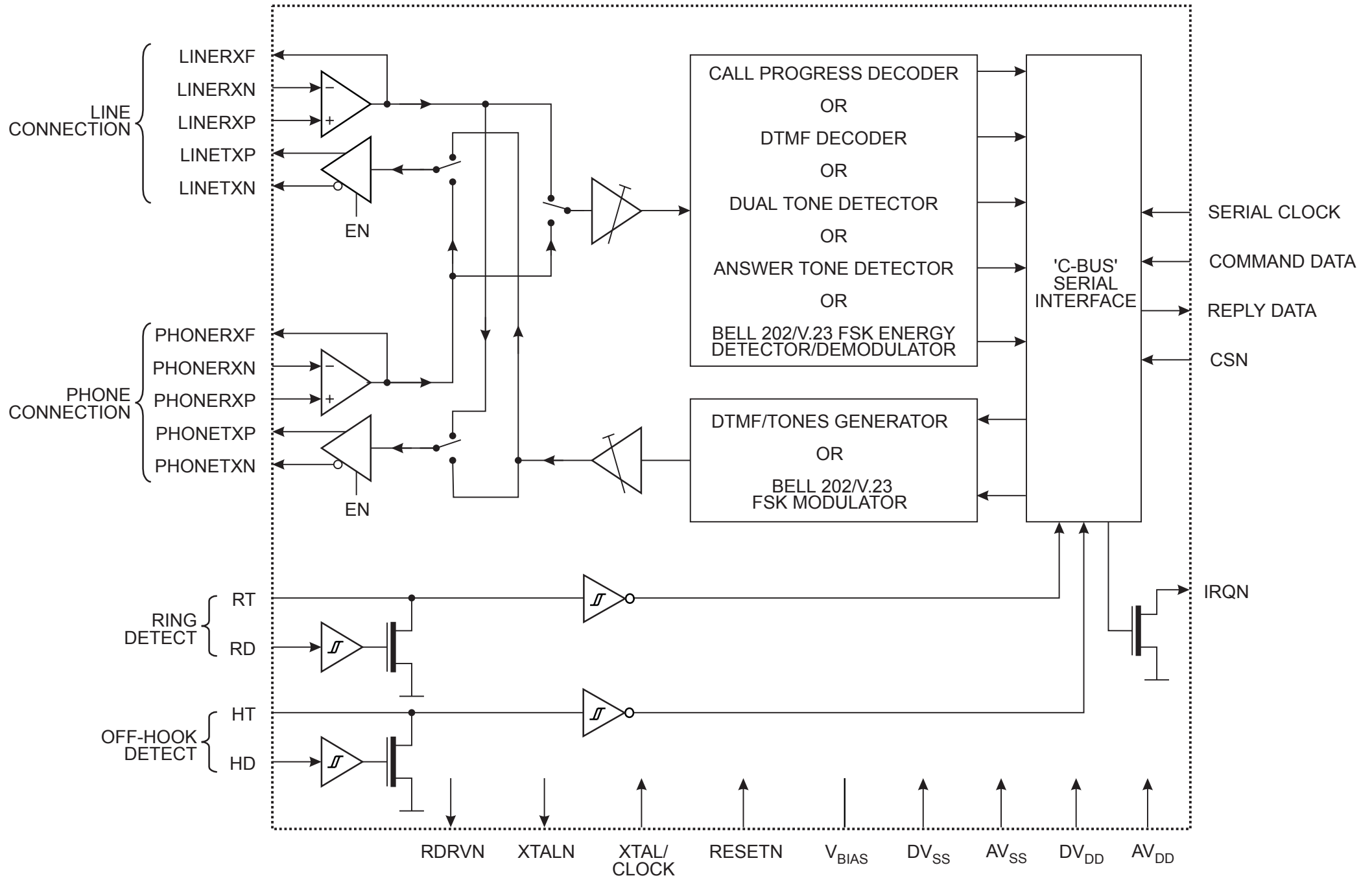
CMX860 Block Diagram
