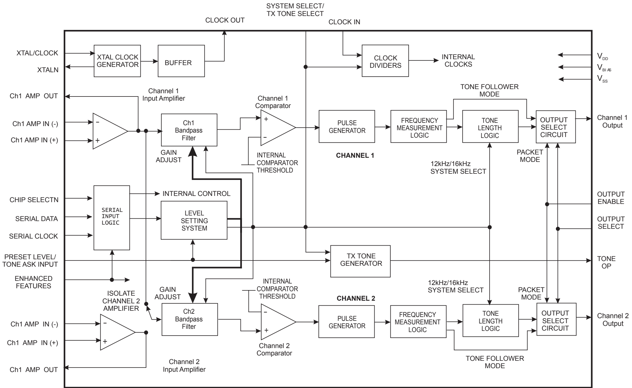
CMX641A Block Diagram
