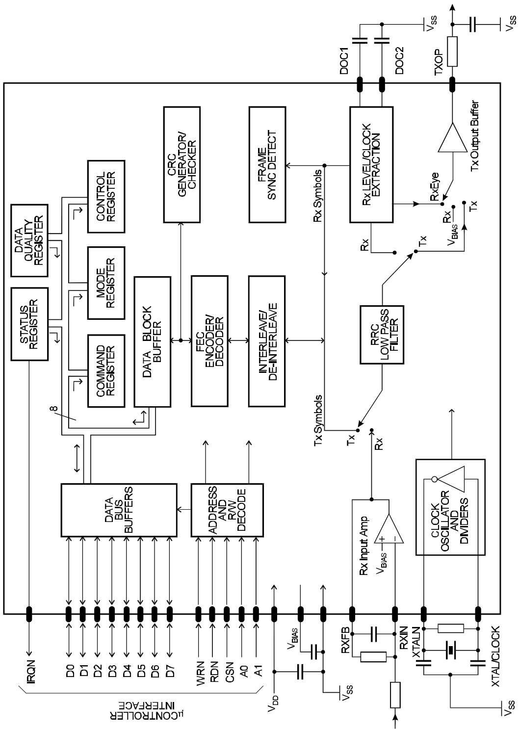
FX/MX919B Block Diagram
