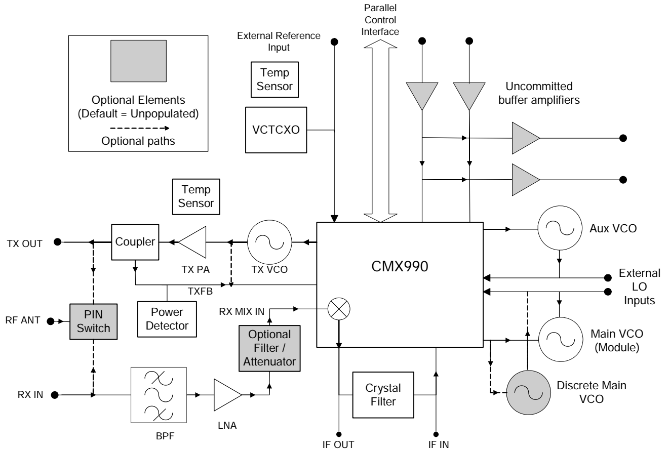
EV990A Block Diagram
