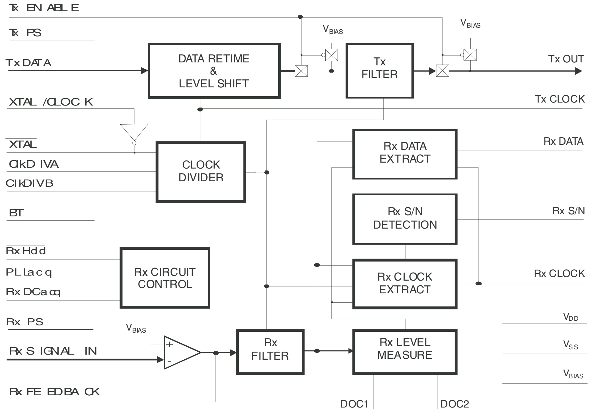
CMX589A Block Diagram
