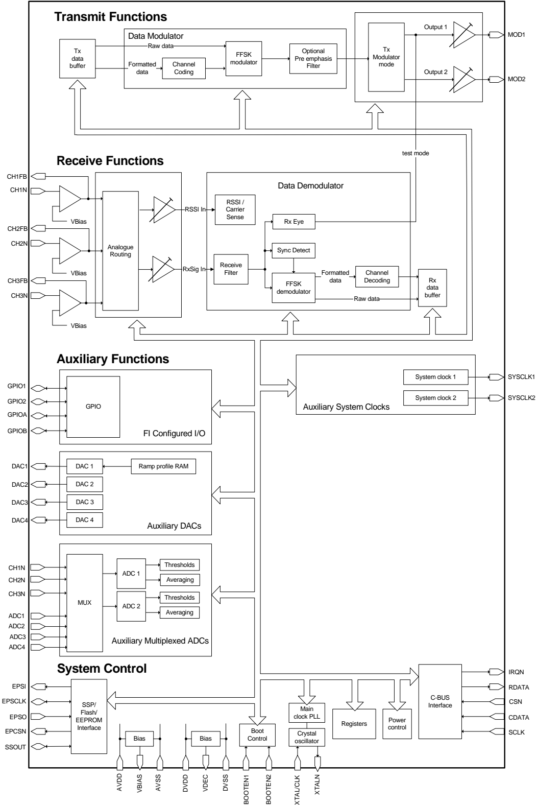
CMX7143 Block Diagram
