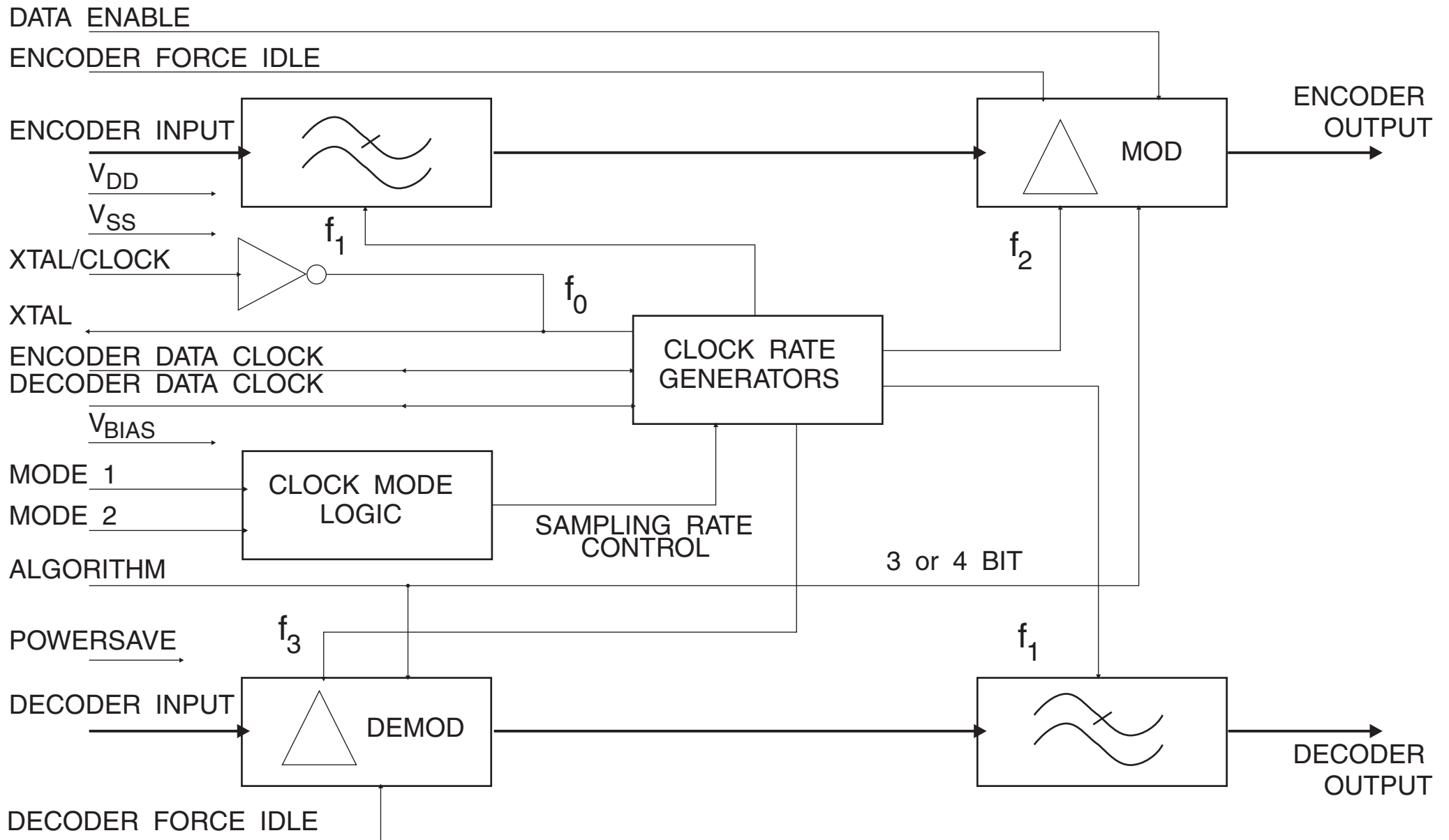
CMX639 Block Diagram
