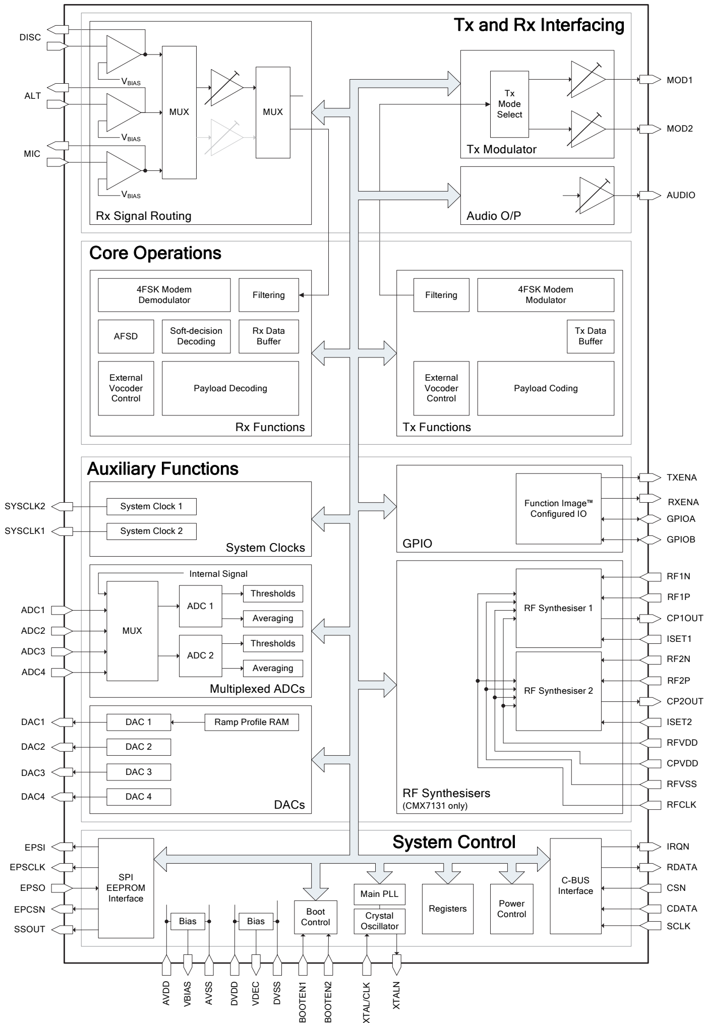
CMX7131/CMX7141 Block Diagram
