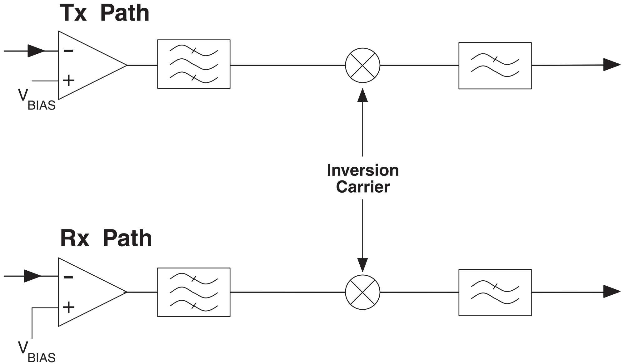
FX/MX128 Block Diagram
