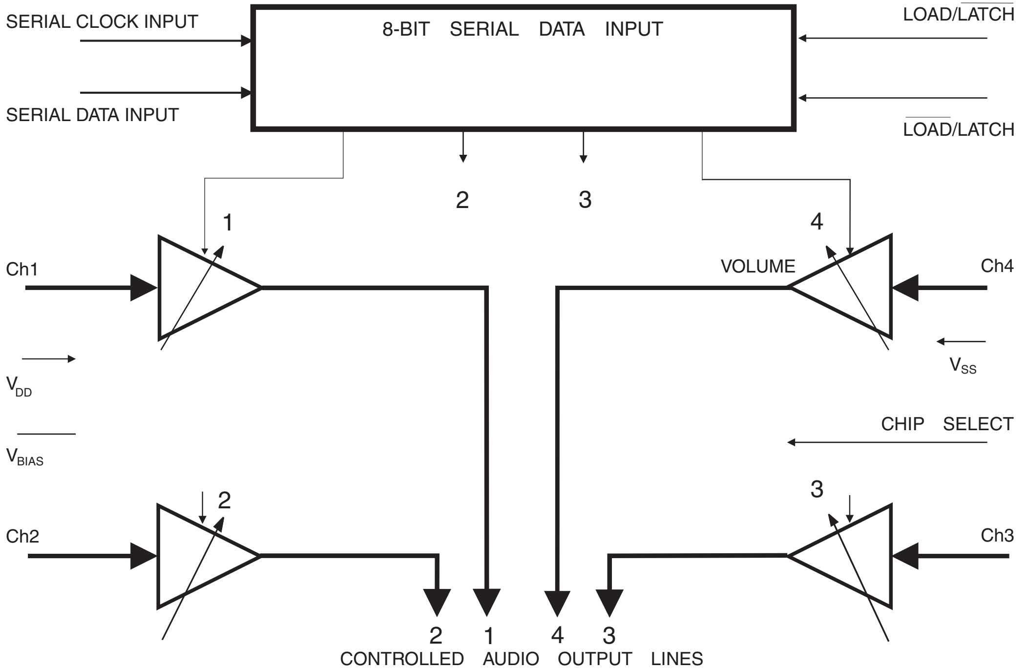
FX/MX019 Block Diagram
